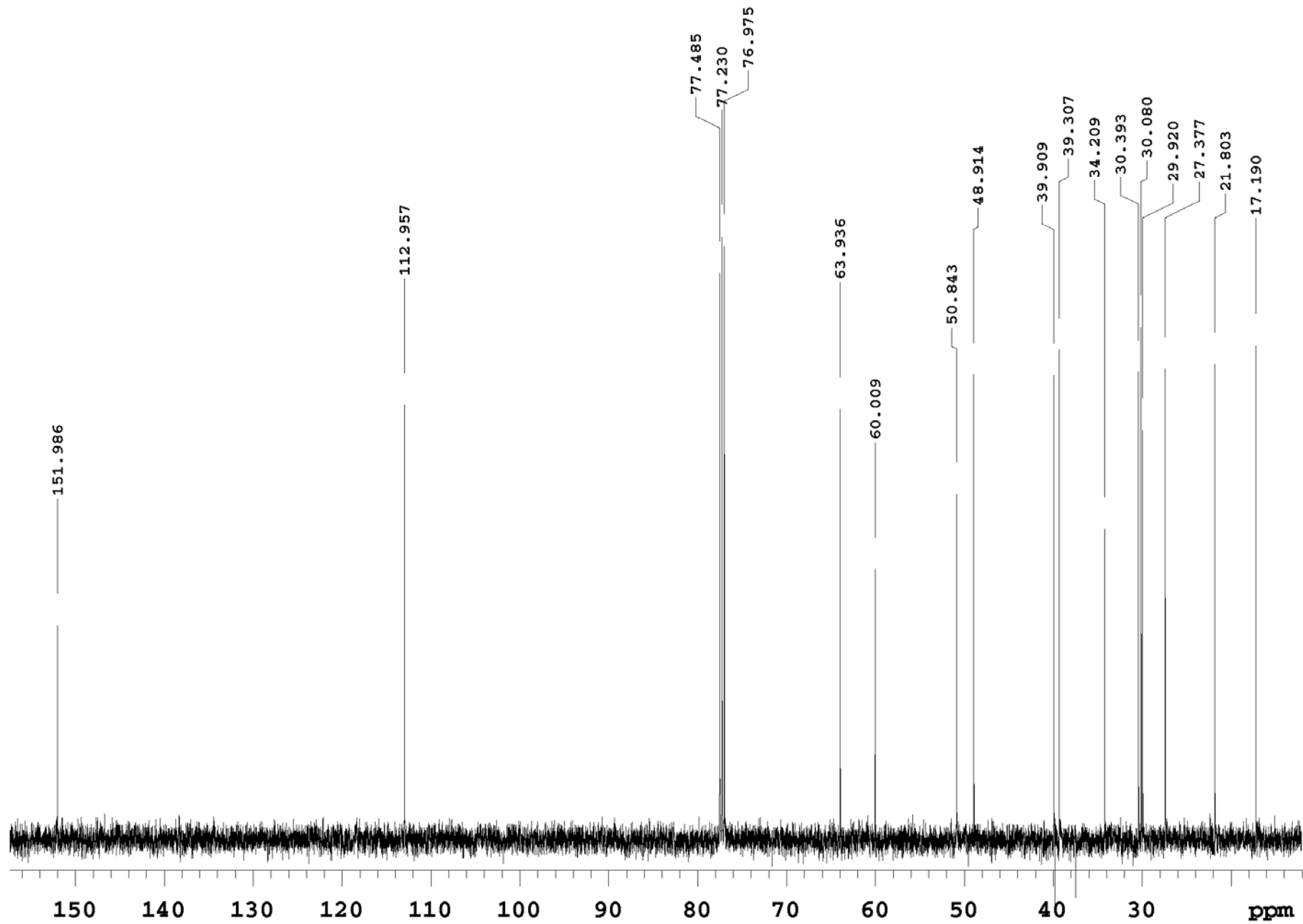
13 C 1-D NMR spectrum of caryophyllene oxide in CDCl 3
