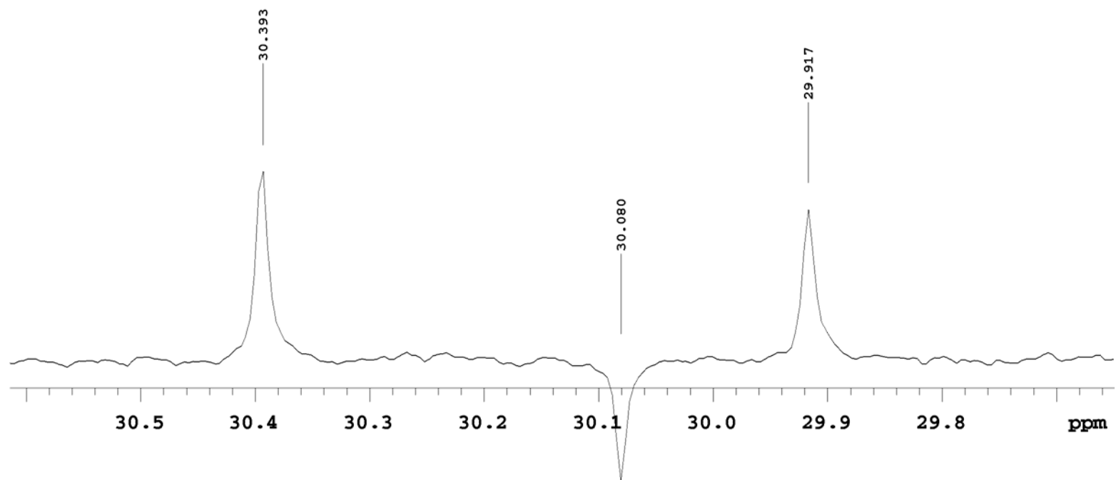
Expansion of ^{13}\text{C} DEPT-135 NMR spectrum of caryophyllene oxide in \text{CDCl}_3
