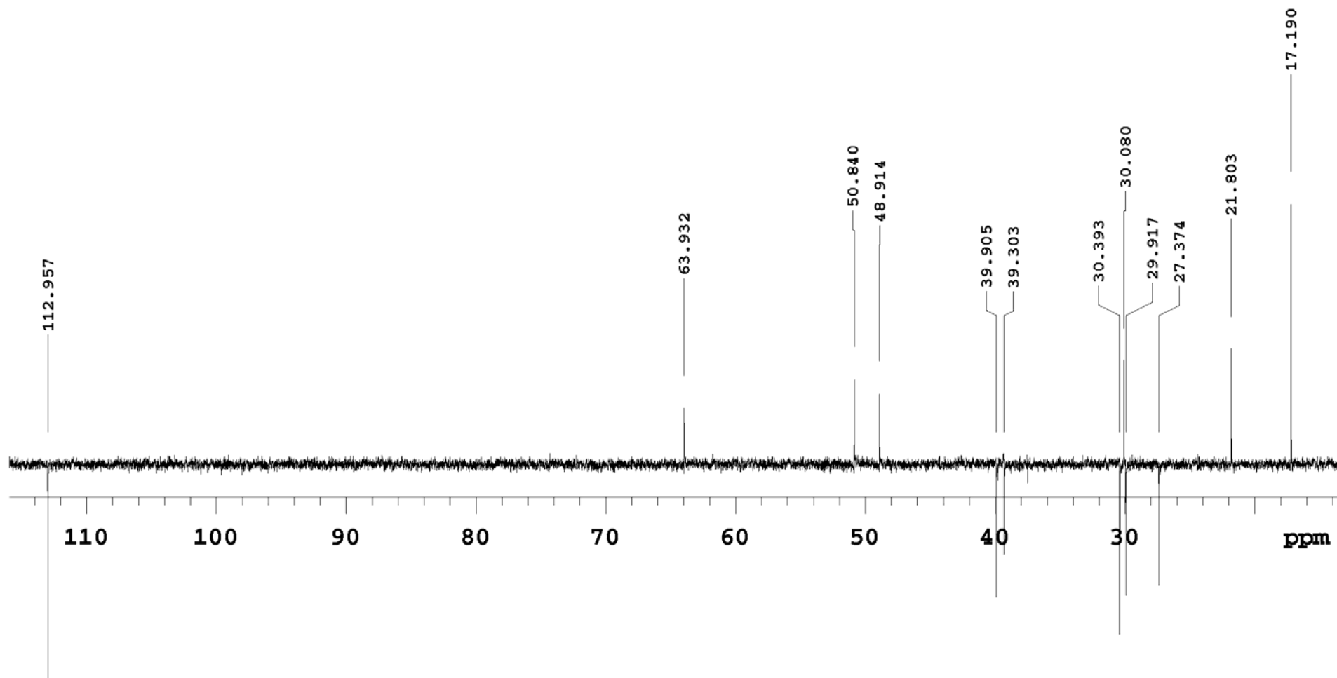
^{13}\text{C} DEPT-135 NMR spectrum of caryophyllene oxide in \text{CDCl}_3
