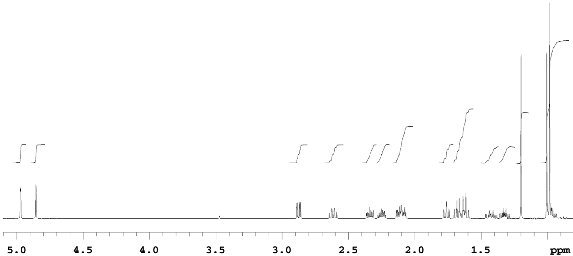
^1\text{H} 1-D NMR spectrum of caryophyllene oxide in \text{CDCl}_3
