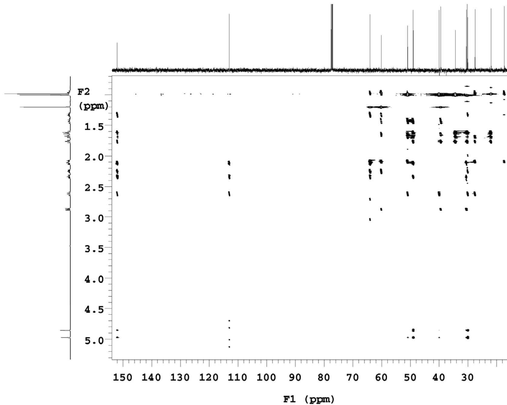
^1\text{H} - ^{13}\text{C} 2-D gHMBC NMR spectrum of caryophyllene oxide in \text{CDCl}_3
