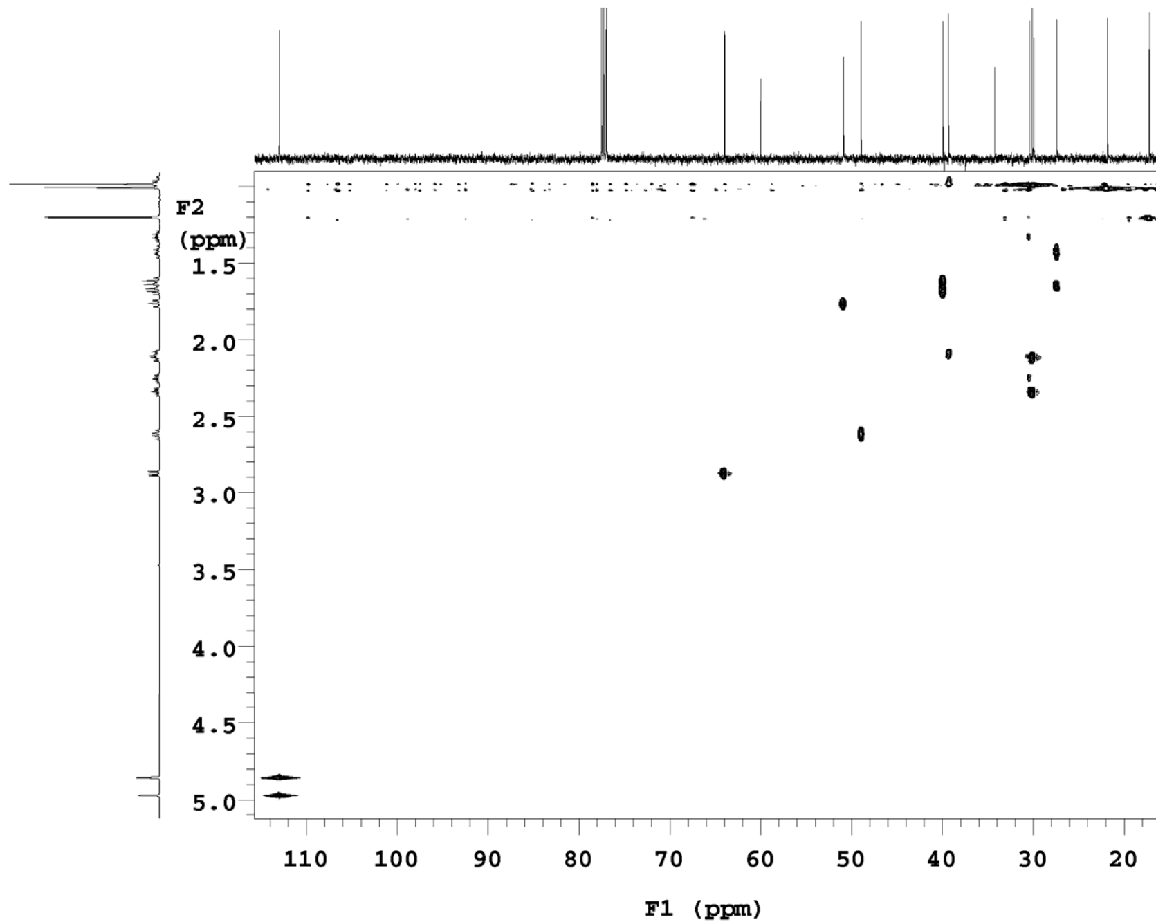
^1\text{H} - ^{13}\text{C} 2-D HSQC NMR spectrum of caryophyllene oxide in \text{CDCl}_3
