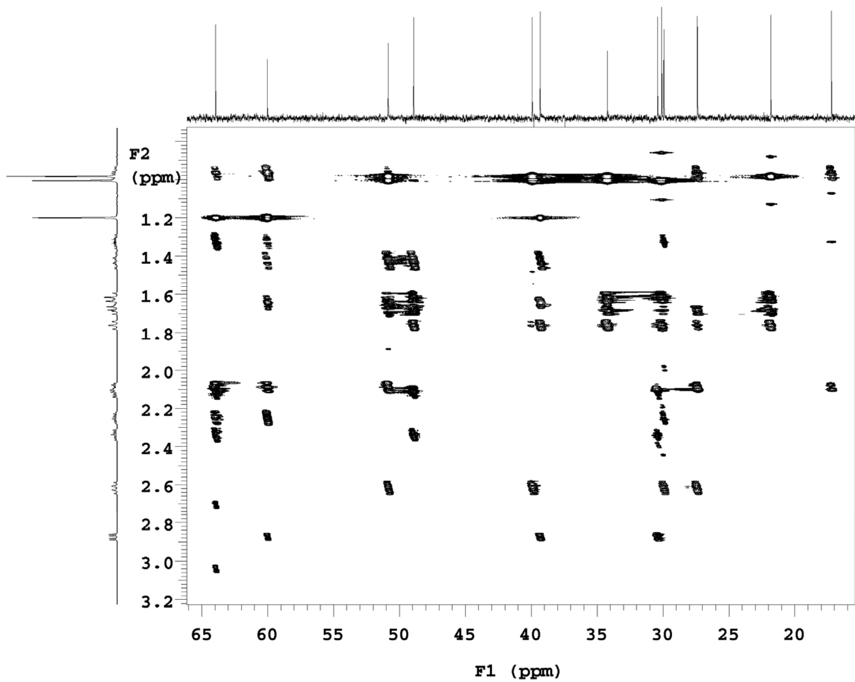
Expansion of ^1\text{H} - ^{13}\text{C} 2-D gHMBC NMR spectrum of caryophyllene oxide in \text{CDCl}_3
