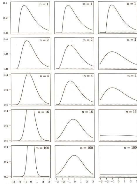
Fig. 14.1. Multiplying the difference \bar{X}_n - \mu of n \text{Gam}(2, 1) random variables. Left column: n^{1/4}(\bar{X}_n - \mu) ; middle column: \sqrt{n}(\bar{X}_n - \mu) ; right column: n(\bar{X}_n - \mu) .
